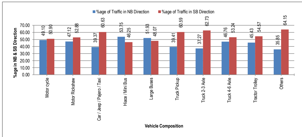
Figure 3-5: Directional Distribution of Traffic Volume at Kamoke (N-5)
