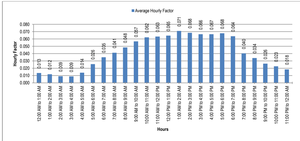
Figure 6-7: Hourly Factor at Sadiqabad (N-5)
