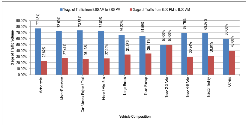
Figure 4-8: Percentage of Traffic Composition in Day and Night Time at Pattoki (N-5)
