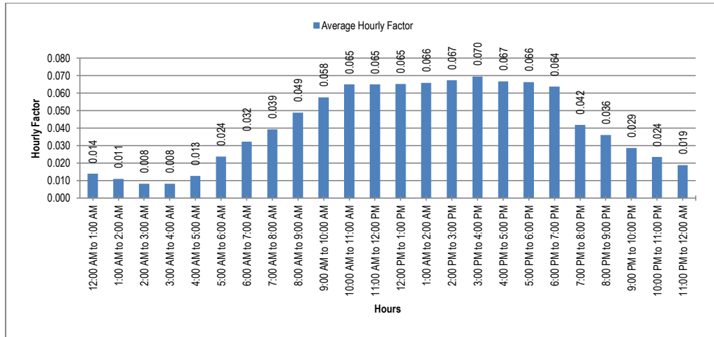
Figure 4-7: Hourly Factor at Pattoki (N-5)
