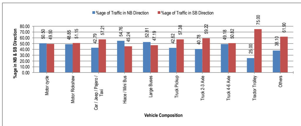
Figure 8-5: Directional Distribution of Traffic Volume at Thatta (N-5)
