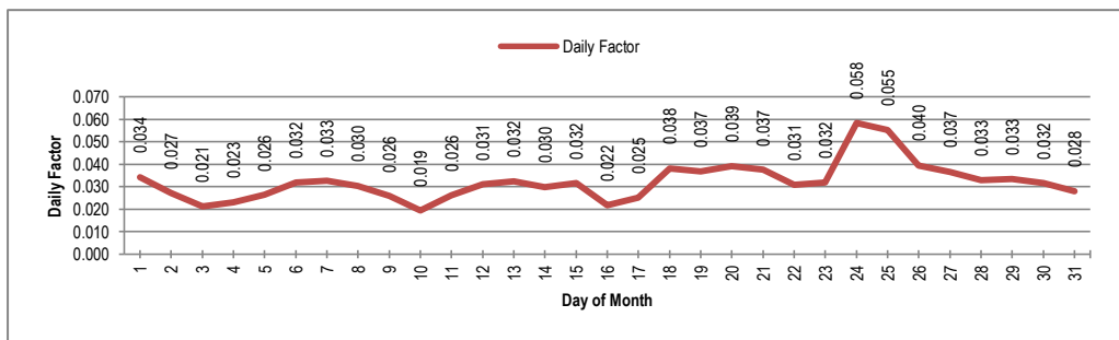
Figure 3-2: Daily Traffic Factor at Kamoke (N-5)
