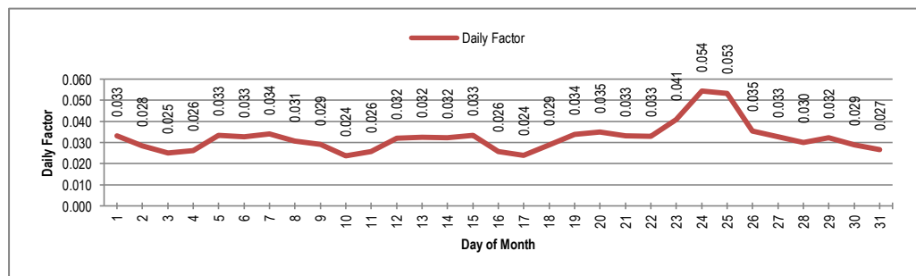
Figure 4-2: Daily Traffic Factor at Pattoki (N-5)
