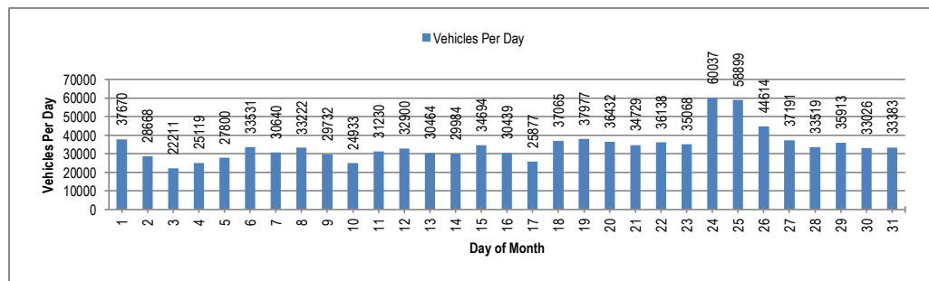
Figure 2-1: Daily Traffic Volume at Jhelum (N-5)
