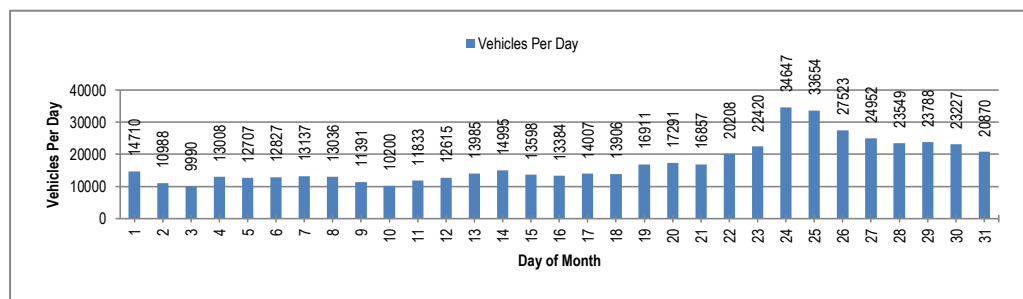
Figure 8-1: Daily Traffic Volume at Thatta (N-5)
