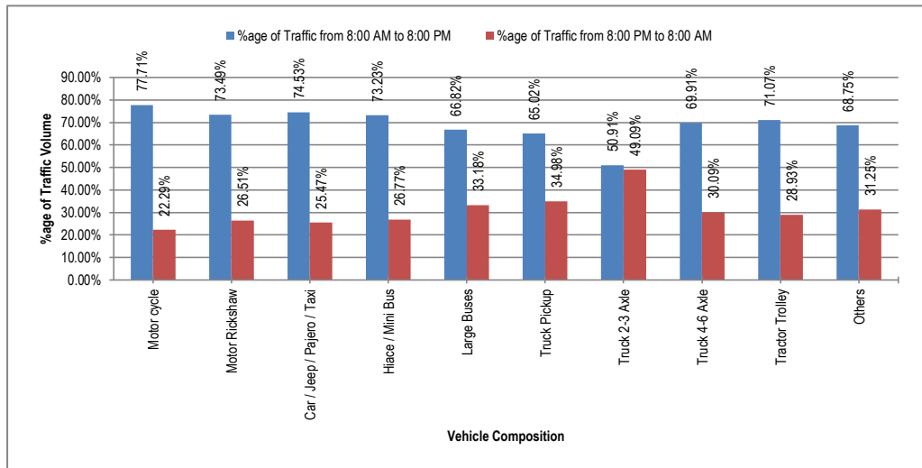
Figure 2-8: Percentage of Traffic Composition in Day and Night Time at Jhelum (N-5)
