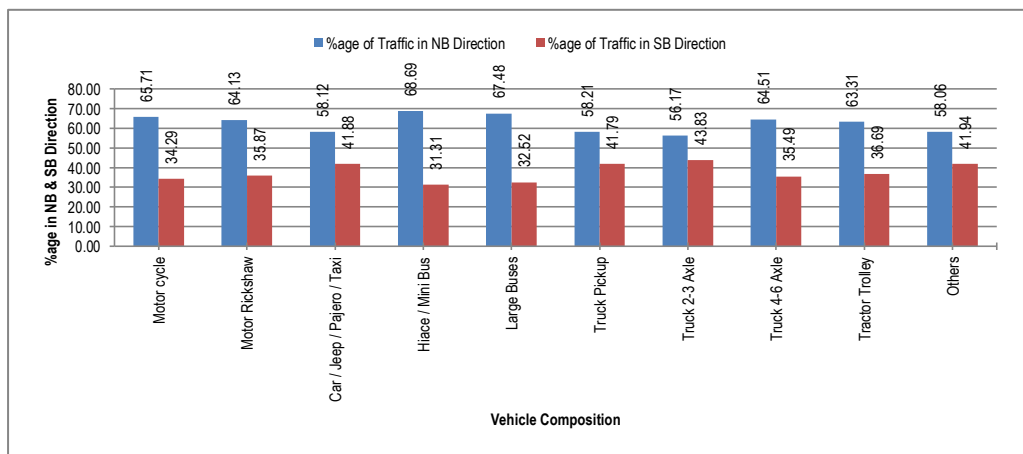
Figure 7-5: Directional Distribution of Traffic Volume at Khairpur (N-5)
