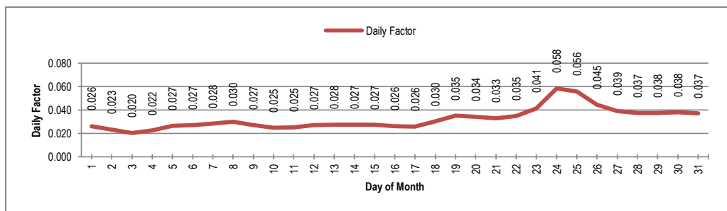
Figure 7-2: Daily Traffic Factor at Khairpur (N-5)
