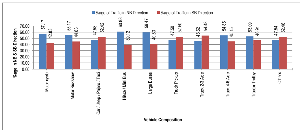
Figure 5-5: Directional Distribution of Traffic Volume at Sutlej (N-5)
