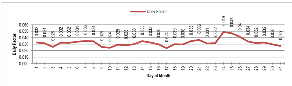
Figure 6-2: Daily Traffic Factor at Sadiqabad (N-5)
