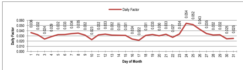
Figure 5-2: Daily Traffic Factor at Sutlej (N-5)
