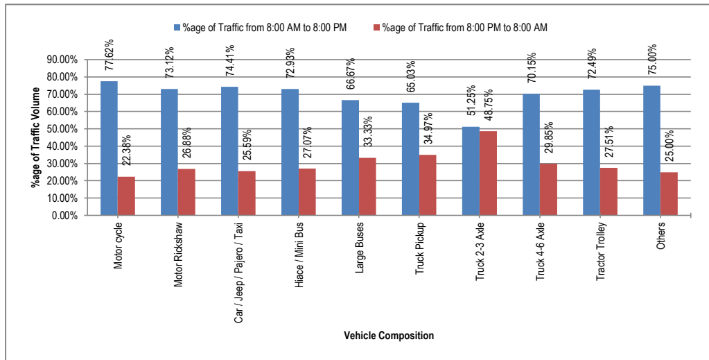
Figure 3-8: Percentage of Traffic Composition in Day and Night Time at Kamoke (N-5)
