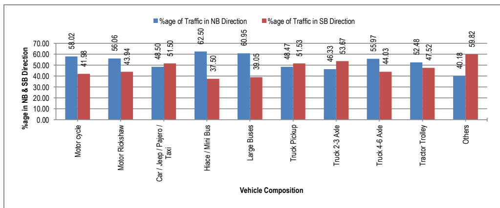
Figure 4-5: Directional Distribution of Traffic Volume at Pattoki (N-5)
