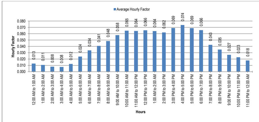
Figure 7-7: Hourly Factor at Khairpur (N-5)
