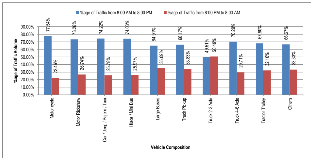
Figure 7-8: Percentage of Traffic Composition in Day and Night Time at Khairpur (N-5)
