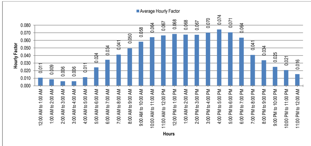
Figure 5-7: Hourly Factor at Sutlej (N-5)
