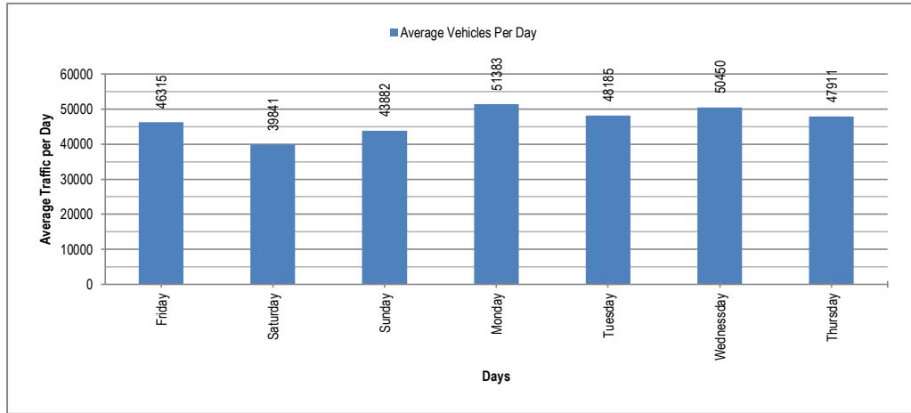
Figure 3-6: Weekly Trend of Traffic at Kamoke (N-5)
