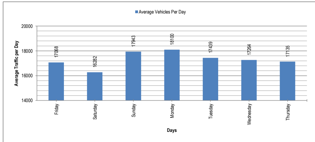
Figure 8-6: Weekly Trend of Traffic at Thatta (N-5)
