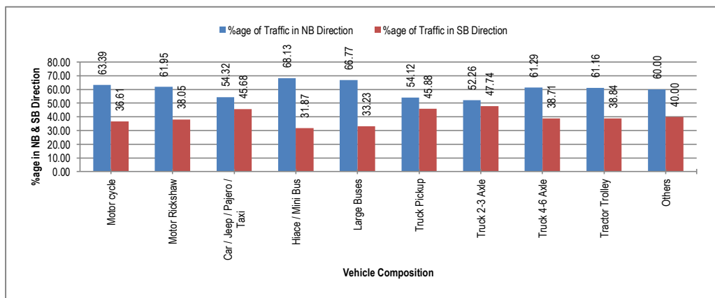
Figure 6-5: Directional Distribution of Traffic Volume at Sadiqabad (N-5)
