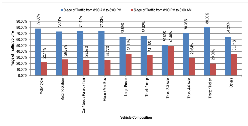
Figure 8-8: Percentage of Traffic Composition in Day and Night Time at Thatta (N-5)
